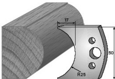
SP-Messer/Blade = Art.-Nr./Item no. 38546 HS-Messer/Blade = Art.-Nr./Item no. 36546 Abweiser/Deflector = Art.-Nr./Item no. 39546
