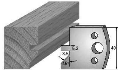
SP-Messer/Blade = Art.-Nr./Item no. 3684 HS-Messer/Blade = Art.-Nr./Item no. 36384 Abweiser/Deflector = Art.-Nr./Item no. 3784
