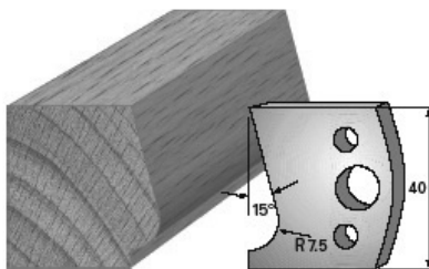
SP-Messer/Blade = Art.-Nr./Item no. 3638 HS-Messer/Blade = Art.-Nr./Item no. 36338 Abweiser/Deflector = Art.-Nr./Item no. 3738
