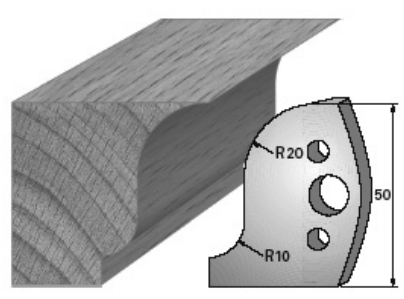
SP-Messer/Blade = Art.-Nr./Item no. 38570 HS-Messer/Blade = Art.-Nr./Item no. 36570 Abweiser/Deflector = Art.-Nr./Item no. 39570
