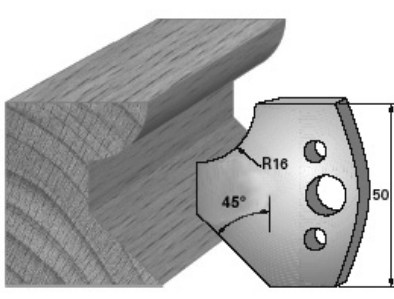
SP-Messer/Blade = Art.-Nr./Item no. 38569 HS-Messer/Blade = Art.-Nr./Item no. 36569 Abweiser/Deflector = Art.-Nr./Item no. 39569
