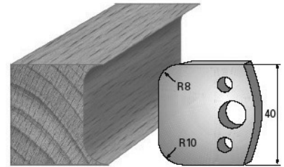
SP-Messer/Blade = Art.-Nr./Item no. 3603 HS-Messer/Blade = Art.-Nr./Item no. 36303 Abweiser/Deflector = Art.-Nr./Item no. 3703
