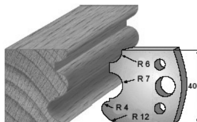
SP-Messer/Blade = Art.-Nr./Item no. 3688 HS-Messer/Blade = Art.-Nr./Item no. 36388 Abweiser/Deflector = Art.-Nr./Item no. 3788
