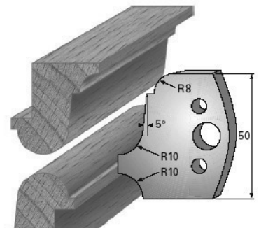
SP-Messer/Blade = Art.-Nr./Item no. 38557 HS-Messer/Blade = Art.-Nr./Item no. 36557 Abweiser/Deflector = Art.-Nr./Item no. 39557
