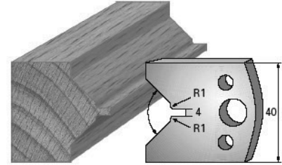
SP-Messer/Blade = Art.-Nr./Item no. 3672 HS-Messer/Blade = Art.-Nr./Item no. 36372 Abweiser/Deflector = Art.-Nr./Item no. 3772
