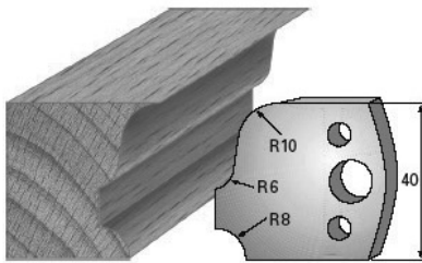
SP-Messer/Blade = Art.-Nr./Item no. 3664 HS-Messer/Blade = Art.-Nr./Item no. 36364 Abweiser/Deflector = Art.-Nr./Item no. 3764
