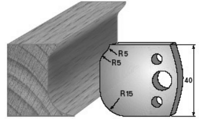
SP-Messer/Blade = Art.-Nr./Item no. 3660 HS-Messer/Blade = Art.-Nr./Item no. 36360 Abweiser/Deflector = Art.-Nr./Item no. 3760
