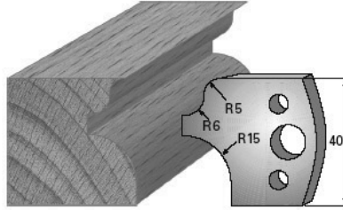
SP-Messer/Blade = Art.-Nr./Item no. 3611 HS-Messer/Blade = Art.-Nr./Item no. 36311 Abweiser/Deflector = Art.-Nr./Item no. 3711
