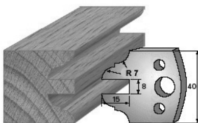
SP-Messer/Blade = Art.-Nr./Item no. 3699 - Konter 4 HS-Messer/Blade = Art.-Nr./Item no. 36399 Abweiser/Deflector = Art.-Nr./Item no. 3799
