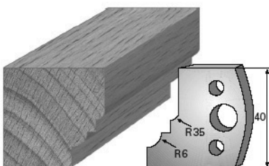
SP-Messer/Blade = Art.-Nr./Item no. 3619 HS-Messer/Blade = Art.-Nr./Item no. 36319 Abweiser/Deflector = Art.-Nr./Item no. 3719
