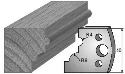
SP-Messer/Blade = Art.-Nr./Item no. 3624 HS-Messer/Blade = Art.-Nr./Item no. 36324 Abweiser/Deflector = Art.-Nr./Item no. 3724
