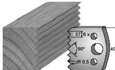
SP-Messer/Blade = Art.-Nr./Item no. 3677 HS-Messer/Blade = Art.-Nr./Item no. 36377 Abweiser/Deflector = Art.-Nr./Item no. 3777
