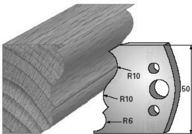
SP-Messer/Blade = Art.-Nr./Item no. 38506 HS-Messer/Blade = Art.-Nr./Item no. 36506 Abweiser/Deflector = Art.-Nr./Item no. 39506
