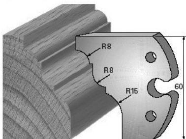
SP-Messer/Blade = Art.-Nr./Item no. 60012 HS-Messer/Blade = Art.-Nr./Item no. 62012 Abweiser/Deflector = Art.-Nr./Item no. 61012
