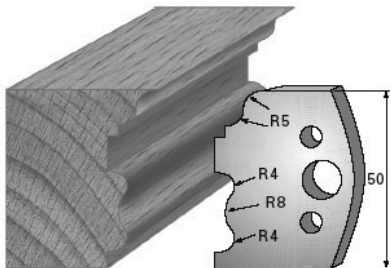
SP-Messer/Blade = Art.-Nr./Item no. 38512 HS-Messer/Blade = Art.-Nr./Item no. 36512 Abweiser/Deflector = Art.-Nr./Item no. 39512
