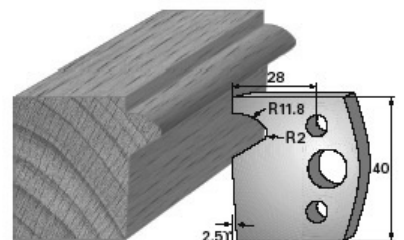
SP-Messer/Blade = Art.-Nr./Item no. 36135 HS-Messer/Blade = Art.-Nr./Item no. 36435 Abweiser/Deflector = Art.-Nr./Item no. 37135
