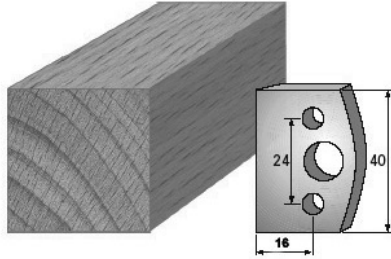
SP-Messer/Blade = Art.-Nr./Item no. 36000 HS-Messer/Blade = Art.-Nr./Item no. 36298 Abweiser/Deflector = Art.-Nr./Item no. 37000
