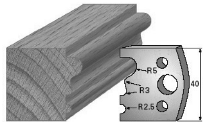
SP-Messer/Blade = Art.-Nr./Item no. 3633 HS-Messer/Blade = Art.-Nr./Item no. 36333 Abweiser/Deflector = Art.-Nr./Item no. 3733
