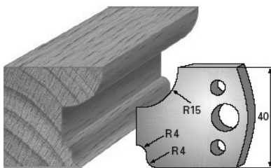
SP-Messer/Blade = Art.-Nr./Item no. 3643 HS-Messer/Blade = Art.-Nr./Item no. 36343 Abweiser/Deflector = Art.-Nr./Item no. 3743
