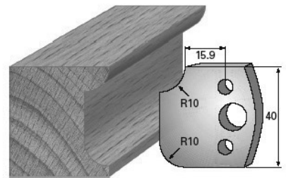
SP-Messer/Blade = Art.-Nr./Item no. 36175 HS-Messer/Blade = Art.-Nr./Item no. 36475 Abweiser/Deflector = Art.-Nr./Item no. 37175
