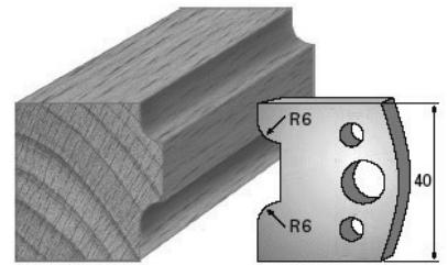
SP-Messer/Blade = Art.-Nr./Item no. 3663 HS-Messer/Blade = Art.-Nr./Item no. 36363 Abweiser/Deflector = Art.-Nr./Item no. 3763
