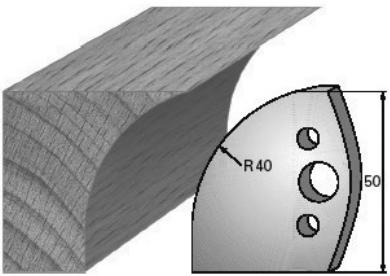
SP-Messer/Blade = Art.-Nr./Item no. 38565 HS-Messer/Blade = Art.-Nr./Item no. 36565 Abweiser/Deflector = Art.-Nr./Item no. 39565
