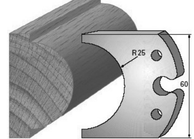
SP-Messer/Blade = Art.-Nr./Item no. 60008 HS-Messer/Blade = Art.-Nr./Item no. 62008 Abweiser/Deflector = Art.-Nr./Item no. 61008
