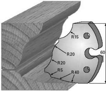
SP-Messer/Blade = Art.-Nr./Item no. 60020 HS-Messer/Blade = Art.-Nr./Item no. 62020 Abweiser/Deflector = Art.-Nr./Item no. 61020
