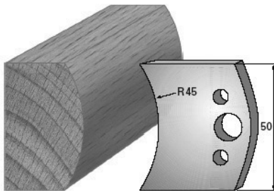
SP-Messer/Blade = Art.-Nr./Item no. 38556 HS-Messer/Blade = Art.-Nr./Item no. 36556 Abweiser/Deflector = Art.-Nr./Item no. 39556
