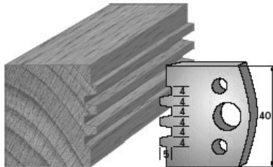
SP-Messer/Blade = Art.-Nr./Item no. 3676 HS-Messer/Blade = Art.-Nr./Item no. 36376 Abweiser/Deflector = Art.-Nr./Item no. 3776
