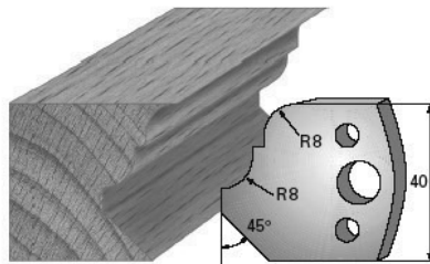
SP-Messer/Blade = Art.-Nr./Item no. 3673 HS-Messer/Blade = Art.-Nr./Item no. 36373 Abweiser/Deflector = Art.-Nr./Item no. 3773
