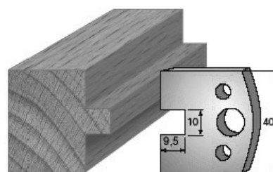
SP-Messer/Blade = Art.-Nr./Item no. 3692 HS-Messer/Blade = Art.-Nr./Item no. 36392 Abweiser/Deflector = Art.-Nr./Item no. 3792
