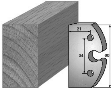
SP-Messer/Blade = Art.-Nr./Item no. 60000 HS-Messer/Blade = Art.-Nr./Item no. 62000 Abweiser/Deflector = Art.-Nr./Item no. 61000
