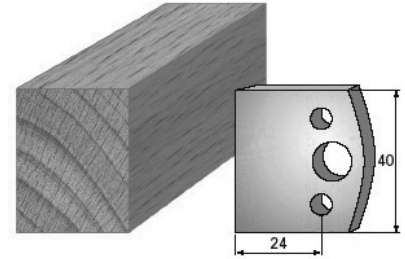
SP-Messer/Blade = Art.-Nr./Item no. 36001 HS-Messer/Blade = Art.-Nr./Item no. 36299 Abweiser/Deflector = Art.-Nr./Item no. 37001
