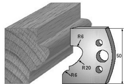
SP-Messer/Blade = Art.-Nr./Item no. 38505 HS-Messer/Blade = Art.-Nr./Item no. 36505 Abweiser/Deflector = Art.-Nr./Item no. 39505
