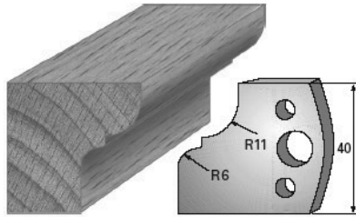
SP-Messer/Blade = Art.-Nr./Item no. 36112 HS-Messer/Blade = Art.-Nr./Item no. 36412 Abweiser/Deflector = Art.-Nr./Item no. 37112
