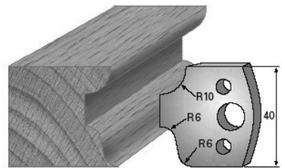
SP-Messer/Blade = Art.-Nr./Item no. 3645 HS-Messer/Blade = Art.-Nr./Item no. 36345 Abweiser/Deflector = Art.-Nr./Item no. 3745
