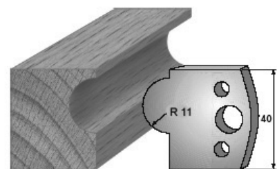
SP-Messer/Blade = Art.-Nr./Item no. 3693 HS-Messer/Blade = Art.-Nr./Item no. 36393 Abweiser/Deflector = Art.-Nr./Item no. 3793
