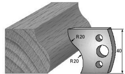
SP-Messer/Blade = Art.-Nr./Item no. 3609 HS-Messer/Blade = Art.-Nr./Item no. 36309 Abweiser/Deflector = Art.-Nr./Item no. 3709
