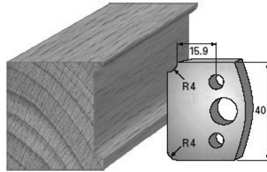
SP-Messer/Blade = Art.-Nr./Item no. 36171 HS-Messer/Blade = Art.-Nr./Item no. 36471 Abweiser/Deflector = Art.-Nr./Item no. 37171
