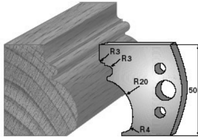
SP-Messer/Blade = Art.-Nr./Item no. 38501 HS-Messer/Blade = Art.-Nr./Item no. 36501 Abweiser/Deflector = Art.-Nr./Item no. 39501
