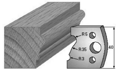
SP-Messer/Blade = Art.-Nr./Item no. 3681 HS-Messer/Blade = Art.-Nr./Item no. 36381 Abweiser/Deflector = Art.-Nr./Item no. 3781
