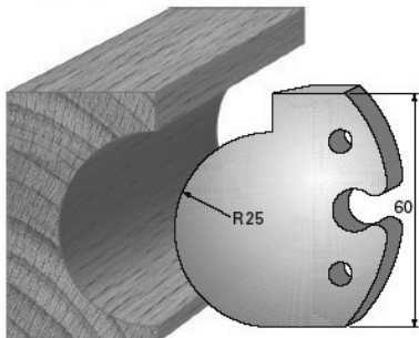
SP-Messer/Blade = Art.-Nr./Item no. 60009 HS-Messer/Blade = Art.-Nr./Item no. 62009 Abweiser/Deflector = Art.-Nr./Item no. 61009
