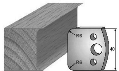
SP-Messer/Blade = Art.-Nr./Item no. 3669 HS-Messer/Blade = Art.-Nr./Item no. 36369 Abweiser/Deflector = Art.-Nr./Item no. 3769
