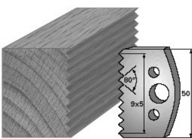
SP-Messer/Blade = Art.-Nr./Item no. 38524 HS-Messer/Blade = Art.-Nr./Item no. 36524 Abweiser/Deflector = Art.-Nr./Item no. 39524
