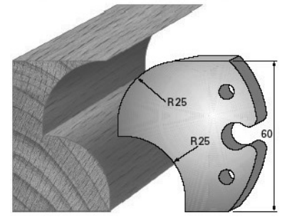
SP-Messer/Blade = Art.-Nr./Item no. 60011 HS-Messer/Blade = Art.-Nr./Item no. 62011 Abweiser/Deflector = Art.-Nr./Item no. 61011
