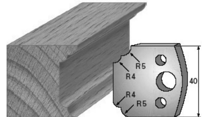
SP-Messer/Blade = Art.-Nr./Item no. 3642 HS-Messer/Blade = Art.-Nr./Item no. 36342 Abweiser/Deflector = Art.-Nr./Item no. 3742
