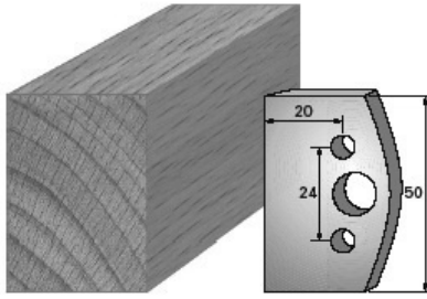
SP-Messer/Blade = Art.-Nr./Item no. 38500 HS-Messer/Blade = Art.-Nr./Item no. 36500 Abweiser/Deflector = Art.-Nr./Item no. 39500
