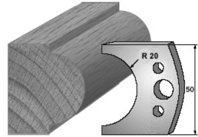
SP-Messer/Blade = Art.-Nr./Item no. 38561 HS-Messer/Blade = Art.-Nr./Item no. 36561 Abweiser/Deflector = Art.-Nr./Item no. 39561
