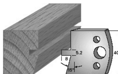
SP-Messer/Blade = Art.-Nr./Item no. 3686 HS-Messer/Blade = Art.-Nr./Item no. 36386 Abweiser/Deflector = Art.-Nr./Item no. 3786
