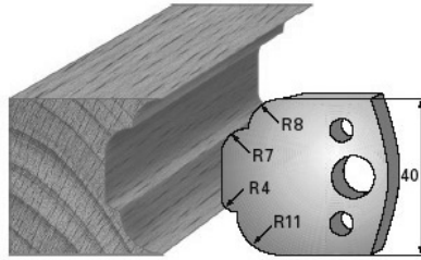
SP-Messer/Blade = Art.-Nr./Item no. 3623 HS-Messer/Blade = Art.-Nr./Item no. 36323 Abweiser/Deflector = Art.-Nr./Item no. 3723
