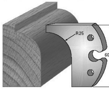
SP-Messer/Blade = Art.-Nr./Item no. 60010 HS-Messer/Blade = Art.-Nr./Item no. 62010 Abweiser/Deflector = Art.-Nr./Item no. 61010
