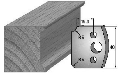
SP-Messer/Blade = Art.-Nr./Item no. 36172 HS-Messer/Blade = Art.-Nr./Item no. 36472 Abweiser/Deflector = Art.-Nr./Item no. 37172
