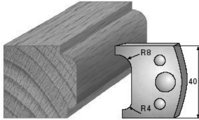
SP-Messer/Blade = Art.-Nr./Item no. 3670 HS-Messer/Blade = Art.-Nr./Item no. 36370 Abweiser/Deflector = Art.-Nr./Item no. 3770
