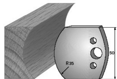
SP-Messer/Blade = Art.-Nr./Item no. 38542 HS-Messer/Blade = Art.-Nr./Item no. 36542 Abweiser/Deflector = Art.-Nr./Item no. 39542
