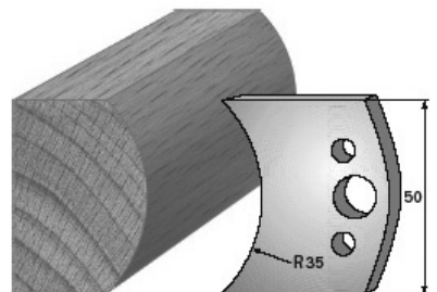
SP-Messer/Blade = Art.-Nr./Item no. 38548 HS-Messer/Blade = Art.-Nr./Item no. 36548 Abweiser/Deflector = Art.-Nr./Item no. 39548
