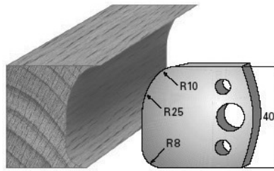
SP-Messer/Blade = Art.-Nr./Item no. 3662 HS-Messer/Blade = Art.-Nr./Item no. 36362 Abweiser/Deflector = Art.-Nr./Item no. 3762
