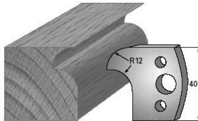
SP-Messer/Blade = Art.-Nr./Item no. 3605 HS-Messer/Blade = Art.-Nr./Item no. 36305 Abweiser/Deflector = Art.-Nr./Item no. 3705
