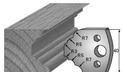
SP-Messer/Blade = Art.-Nr./Item no. 3621 HS-Messer/Blade = Art.-Nr./Item no. 36321 Abweiser/Deflector = Art.-Nr./Item no. 3721
