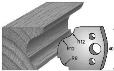
SP-Messer/Blade = Art.-Nr./Item no. 3661 HS-Messer/Blade = Art.-Nr./Item no. 36361 Abweiser/Deflector = Art.-Nr./Item no. 3761
