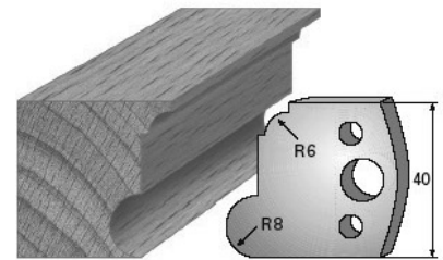
SP-Messer/Blade = Art.-Nr./Item no. 3654 HS-Messer/Blade = Art.-Nr./Item no. 36354 Abweiser/Deflector = Art.-Nr./Item no. 3754
