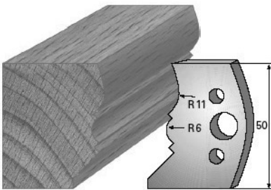
SP-Messer/Blade = Art.-Nr./Item no. 38503 HS-Messer/Blade = Art.-Nr./Item no. 36503 Abweiser/Deflector = Art.-Nr./Item no. 39503
