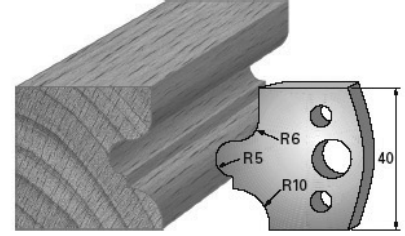
SP-Messer/Blade = Art.-Nr./Item no. 3612 HS-Messer/Blade = Art.-Nr./Item no. 36312 Abweiser/Deflector = Art.-Nr./Item no. 3712
