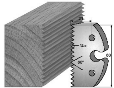
SP-Messer/Blade = Art.-Nr./Item no. 60003 HS-Messer/Blade = Art.-Nr./Item no. 62003 Abweiser/Deflector = Art.-Nr./Item no. 61003
