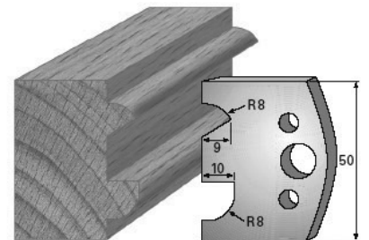
SP-Messer/Blade = Art.-Nr./Item no. 38514 HS-Messer/Blade = Art.-Nr./Item no. 36514 Abweiser/Deflector = Art.-Nr./Item no. 39514
