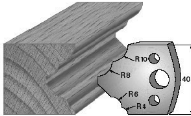
SP-Messer/Blade = Art.-Nr./Item no. 36125 HS-Messer/Blade = Art.-Nr./Item no. 36425 Abweiser/Deflector = Art.-Nr./Item no. 37125
