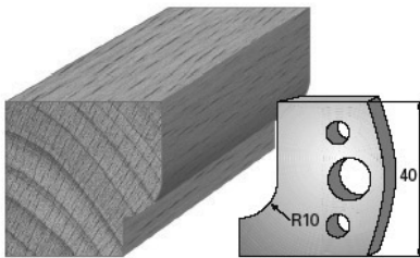
SP-Messer/Blade = Art.-Nr./Item no. 3613 HS-Messer/Blade = Art.-Nr./Item no. 36313 Abweiser/Deflector = Art.-Nr./Item no. 3713
