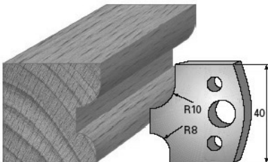
SP-Messer/Blade = Art.-Nr./Item no. 3640 HS-Messer/Blade = Art.-Nr./Item no. 36340 Abweiser/Deflector = Art.-Nr./Item no. 3740
