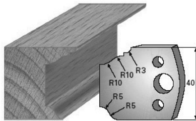
SP-Messer/Blade = Art.-Nr./Item no. 3679 HS-Messer/Blade = Art.-Nr./Item no. 36379 Abweiser/Deflector = Art.-Nr./Item no. 3779
