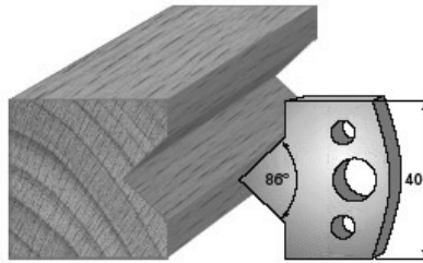
SP-Messer/Blade = Art.-Nr./Item no. 3635 HS-Messer/Blade = Art.-Nr./Item no. 36335 Abweiser/Deflector = Art.-Nr./Item no. 3735
