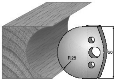
SP-Messer/Blade = Art.-Nr./Item no. 38524 HS-Messer/Blade = Art.-Nr./Item no. 36524 Abweiser/Deflector = Art.-Nr./Item no. 39524
