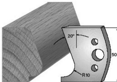
SP-Messer/Blade = Art.-Nr./Item no. 38575 HS-Messer/Blade = Art.-Nr./Item no. 36575 Abweiser/Deflector = Art.-Nr./Item no. 39575
