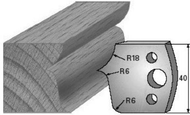
SP-Messer/Blade = Art.-Nr./Item no. 3646 HS-Messer/Blade = Art.-Nr./Item no. 36346 Abweiser/Deflector = Art.-Nr./Item no. 3746
