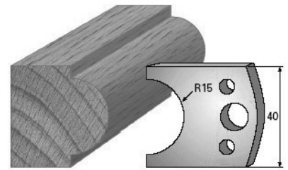
SP-Messer/Blade = Art.-Nr./Item no. 3666 HS-Messer/Blade = Art.-Nr./Item no. 36366 Abweiser/Deflector = Art.-Nr./Item no. 3766
