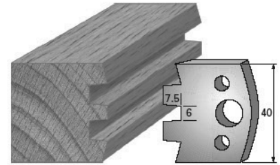
SP-Messer/Blade = Art.-Nr./Item no. 36114 HS-Messer/Blade = Art.-Nr./Item no. 36414 Abweiser/Deflector = Art.-Nr./Item no. 37114
