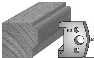
SP-Messer/Blade = Art.-Nr./Item no. 3632 HS-Messer/Blade = Art.-Nr./Item no. 36332 Abweiser/Deflector = Art.-Nr./Item no. 3732
