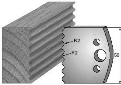
SP-Messer/Blade = Art.-Nr./Item no. 38552 HS-Messer/Blade = Art.-Nr./Item no. 36552 Abweiser/Deflector = Art.-Nr./Item no. 39552
