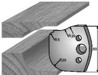
SP-Messer/Blade = Art.-Nr./Item no. 38577 HS-Messer/Blade = Art.-Nr./Item no. 36577 Abweiser/Deflector = Art.-Nr./Item no. 39577
