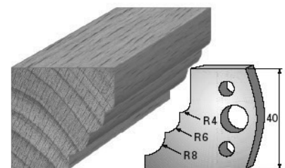
SP-Messer/Blade = Art.-Nr./Item no. 36132 HS-Messer/Blade = Art.-Nr./Item no. 36432 Abweiser/Deflector = Art.-Nr./Item no. 37132
