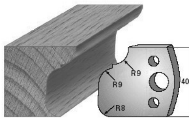
SP-Messer/Blade = Art.-Nr./Item no. 3668 HS-Messer/Blade = Art.-Nr./Item no. 36368 Abweiser/Deflector = Art.-Nr./Item no. 3768
