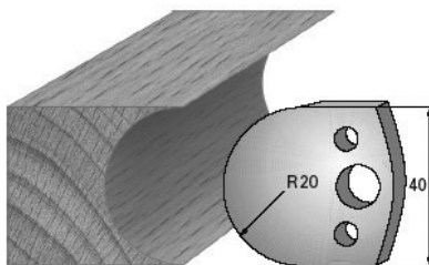
SP-Messer/Blade = Art.-Nr./Item no. 36131 HS-Messer/Blade = Art.-Nr./Item no. 36431 Abweiser/Deflector = Art.-Nr./Item no. 37131
