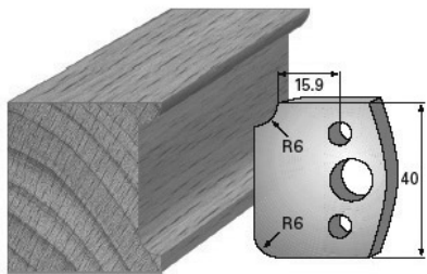
SP-Messer/Blade = Art.-Nr./Item no. 36173 HS-Messer/Blade = Art.-Nr./Item no. 36473 Abweiser/Deflector = Art.-Nr./Item no. 37173
