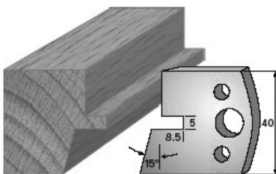
SP-Messer/Blade = Art.-Nr./Item no. 3685 HS-Messer/Blade = Art.-Nr./Item no. 36385 Abweiser/Deflector = Art.-Nr./Item no. 3785
