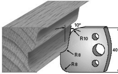
SP-Messer/Blade = Art.-Nr./Item no. 3659 HS-Messer/Blade = Art.-Nr./Item no. 36359 Abweiser/Deflector = Art.-Nr./Item no. 3759
