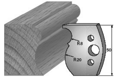
SP-Messer/Blade = Art.-Nr./Item no. 38502 HS-Messer/Blade = Art.-Nr./Item no. 36502 Abweiser/Deflector = Art.-Nr./Item no. 39502
