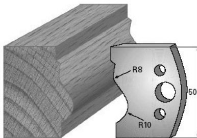
SP-Messer/Blade = Art.-Nr./Item no. 38510 HS-Messer/Blade = Art.-Nr./Item no. 36510 Abweiser/Deflector = Art.-Nr./Item no. 39510
