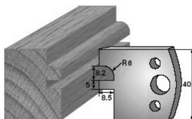
SP-Messer/Blade = Art.-Nr./Item no. 36134 HS-Messer/Blade = Art.-Nr./Item no. 36434 Abweiser/Deflector = Art.-Nr./Item no. 37134
