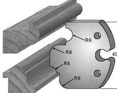
SP-Messer/Blade = Art.-Nr./Item no. 60006 HS-Messer/Blade = Art.-Nr./Item no. 62006 Abweiser/Deflector = Art.-Nr./Item no. 61006
