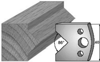
SP-Messer/Blade = Art.-Nr./Item no. 3634 HS-Messer/Blade = Art.-Nr./Item no. 36334 Abweiser/Deflector = Art.-Nr./Item no. 3734
