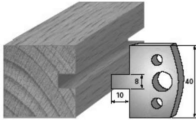
SP-Messer/Blade = Art.-Nr./Item no. 3694 HS-Messer/Blade = Art.-Nr./Item no. 36394 Abweiser/Deflector = Art.-Nr./Item no. 3794
