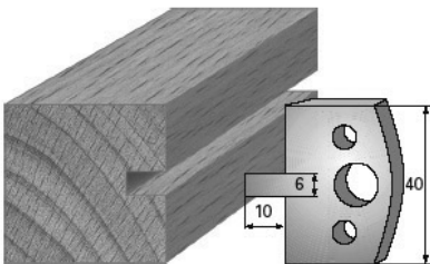
SP-Messer/Blade = Art.-Nr./Item no. 3616 HS-Messer/Blade = Art.-Nr./Item no. 36316 Abweiser/Deflector = Art.-Nr./Item no. 3716
