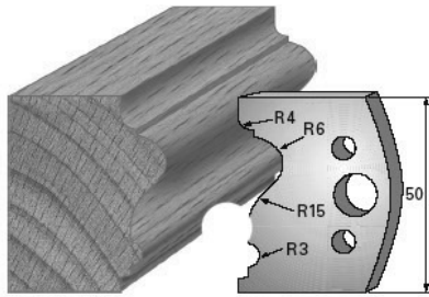
SP-Messer/Blade = Art.-Nr./Item no. 38512 HS-Messer/Blade = Art.-Nr./Item no. 36512 Abweiser/Deflector = Art.-Nr./Item no. 39512
