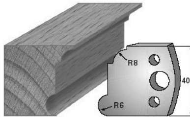
SP-Messer/Blade = Art.-Nr./Item no. 3653 HS-Messer/Blade = Art.-Nr./Item no. 36353 Abweiser/Deflector = Art.-Nr./Item no. 3753
