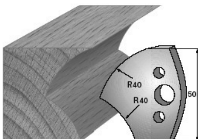
SP-Messer/Blade = Art.-Nr./Item no. 38550 HS-Messer/Blade = Art.-Nr./Item no. 36550 Abweiser/Deflector = Art.-Nr./Item no. 39550
