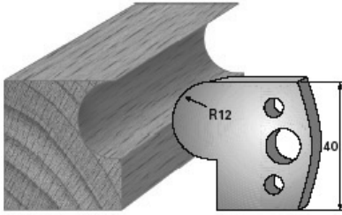
SP-Messer/Blade = Art.-Nr./Item no. 3658 HS-Messer/Blade = Art.-Nr./Item no. 36358 Abweiser/Deflector = Art.-Nr./Item no. 3758
