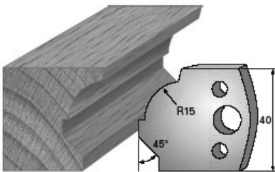
SP-Messer/Blade = Art.-Nr./Item no. 3637 HS-Messer/Blade = Art.-Nr./Item no. 36337 Abweiser/Deflector = Art.-Nr./Item no. 3737
