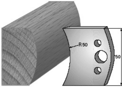
SP-Messer/Blade = Art.-Nr./Item no. 38559 HS-Messer/Blade = Art.-Nr./Item no. 36559 Abweiser/Deflector = Art.-Nr./Item no. 39559
