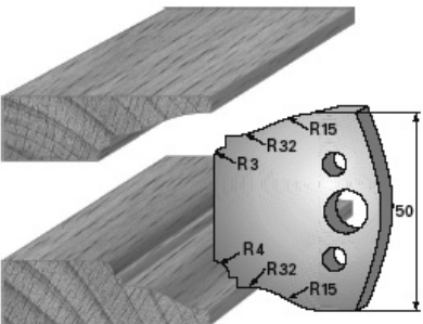
SP-Messer/Blade = Art.-Nr./Item no. 38568 HS-Messer/Blade = Art.-Nr./Item no. 36568 Abweiser/Deflector = Art.-Nr./Item no. 39568
