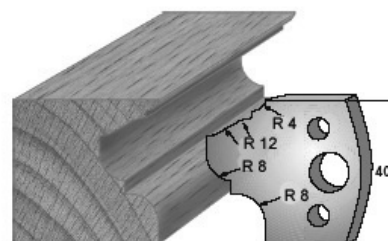
SP-Messer/Blade = Art.-Nr./Item no. 3689 HS-Messer/Blade = Art.-Nr./Item no. 36389 Abweiser/Deflector = Art.-Nr./Item no. 3789
