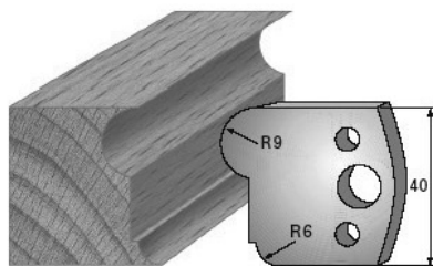
SP-Messer/Blade = Art.-Nr./Item no. 3655 HS-Messer/Blade = Art.-Nr./Item no. 36355 Abweiser/Deflector = Art.-Nr./Item no. 3755
