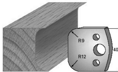
SP-Messer/Blade = Art.-Nr./Item no. 3650 HS-Messer/Blade = Art.-Nr./Item no. 36350 Abweiser/Deflector = Art.-Nr./Item no. 3750
