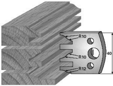
SP-Messer/Blade = Art.-Nr./Item no. 36124 HS-Messer/Blade = Art.-Nr./Item no. 36424 Abweiser/Deflector = Art.-Nr./Item no. 37124
