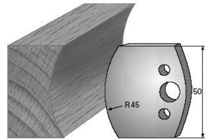
SP-Messer/Blade = Art.-Nr./Item no. 38554 HS-Messer/Blade = Art.-Nr./Item no. 36554 Abweiser/Deflector = Art.-Nr./Item no. 39554
