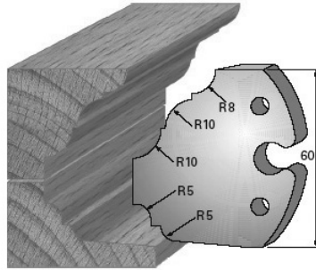
SP-Messer/Blade = Art.-Nr./Item no. 60021 HS-Messer/Blade = Art.-Nr./Item no. 62021 Abweiser/Deflector = Art.-Nr./Item no. 61021
