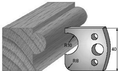
SP-Messer/Blade = Art.-Nr./Item no. 3604 HS-Messer/Blade = Art.-Nr./Item no. 36304 Abweiser/Deflector = Art.-Nr./Item no. 3704
