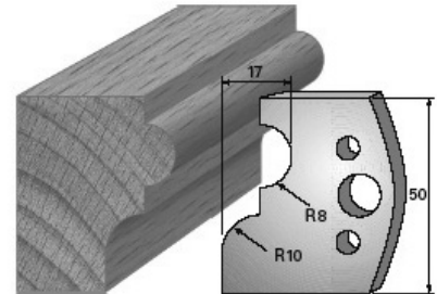
SP-Messer/Blade = Art.-Nr./Item no. 38551 HS-Messer/Blade = Art.-Nr./Item no. 36551 Abweiser/Deflector = Art.-Nr./Item no. 39551
