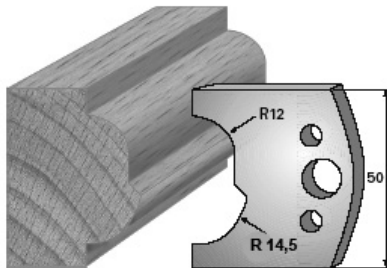
SP-Messer/Blade = Art.-Nr./Item no. 38519 HS-Messer/Blade = Art.-Nr./Item no. 36519 Abweiser/Deflector = Art.-Nr./Item no. 39519
