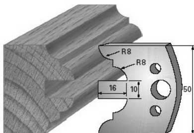
SP-Messer/Blade = Art.-Nr./Item no. 38522 HS-Messer/Blade = Art.-Nr./Item no. 36522 Abweiser/Deflector = Art.-Nr./Item no. 39522
