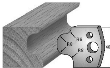
SP-Messer/Blade = Art.-Nr./Item no. 3656 HS-Messer/Blade = Art.-Nr./Item no. 36356 Abweiser/Deflector = Art.-Nr./Item no. 3756
