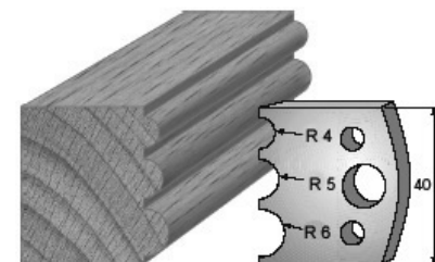
SP-Messer/Blade = Art.-Nr./Item no. 3690 HS-Messer/Blade = Art.-Nr./Item no. 36390 Abweiser/Deflector = Art.-Nr./Item no. 3790
