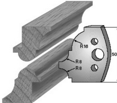
SP-Messer/Blade = Art.-Nr./Item no. 38541 HS-Messer/Blade = Art.-Nr./Item no. 36541 Abweiser/Deflector = Art.-Nr./Item no. 39541
