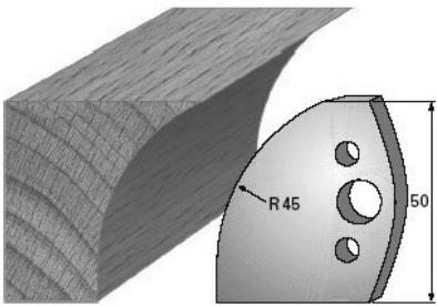
SP-Messer/Blade = Art.-Nr./Item no. 38566 HS-Messer/Blade = Art.-Nr./Item no. 36566 Abweiser/Deflector = Art.-Nr./Item no. 39566
