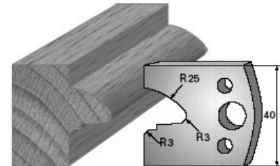
SP-Messer/Blade = Art.-Nr./Item no. 3678 HS-Messer/Blade = Art.-Nr./Item no. 36378 Abweiser/Deflector = Art.-Nr./Item no. 3778
