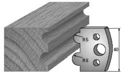
SP-Messer/Blade = Art.-Nr./Item no. 3630 HS-Messer/Blade = Art.-Nr./Item no. 36330 Abweiser/Deflector = Art.-Nr./Item no. 3730
