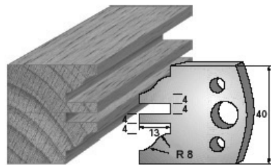
SP-Messer/Blade = Art.-Nr./Item no. 3697 - Konter 2 HS-Messer/Blade = Art.-Nr./Item no. 36397 Abweiser/Deflector = Art.-Nr./Item no. 3797
