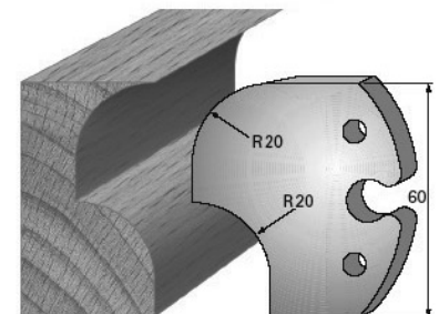
SP-Messer/Blade = Art.-Nr./Item no. 60019 HS-Messer/Blade = Art.-Nr./Item no. 62019 Abweiser/Deflector = Art.-Nr./Item no. 61019
