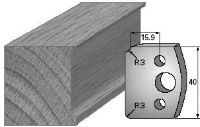
SP-Messer/Blade = Art.-Nr./Item no. 36170 HS-Messer/Blade = Art.-Nr./Item no. 36470 Abweiser/Deflector = Art.-Nr./Item no. 37170
