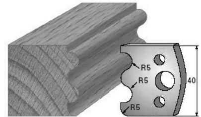
SP-Messer/Blade = Art.-Nr./Item no. 3606 HS-Messer/Blade = Art.-Nr./Item no. 36306 Abweiser/Deflector = Art.-Nr./Item no. 3706
