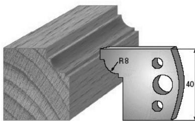
SP-Messer/Blade = Art.-Nr./Item no. 3667 HS-Messer/Blade = Art.-Nr./Item no. 36367 Abweiser/Deflector = Art.-Nr./Item no. 3767
