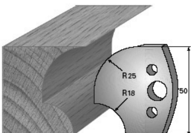
SP-Messer/Blade = Art.-Nr./Item no. 38549 HS-Messer/Blade = Art.-Nr./Item no. 36549 Abweiser/Deflector = Art.-Nr./Item no. 39549
