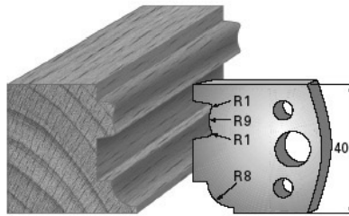
SP-Messer/Blade = Art.-Nr./Item no. 3626 HS-Messer/Blade = Art.-Nr./Item no. 36326 Abweiser/Deflector = Art.-Nr./Item no. 3726
