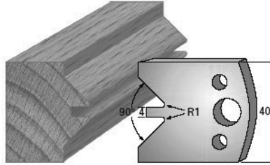
SP-Messer/Blade = Art.-Nr./Item no. 3671 HS-Messer/Blade = Art.-Nr./Item no. 36371 Abweiser/Deflector = Art.-Nr./Item no. 3771
