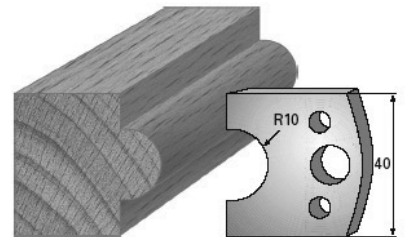
SP-Messer/Blade = Art.-Nr./Item no. 3615 HS-Messer/Blade = Art.-Nr./Item no. 36315 Abweiser/Deflector = Art.-Nr./Item no. 3715
