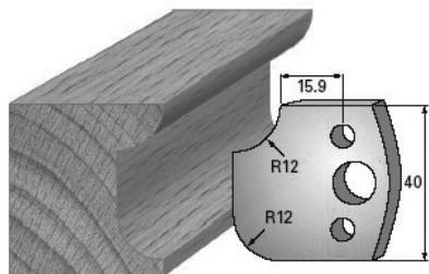
SP-Messer/Blade = Art.-Nr./Item no. 36176 HS-Messer/Blade = Art.-Nr./Item no. 36476 Abweiser/Deflector = Art.-Nr./Item no. 37176
