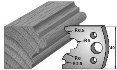
SP-Messer/Blade = Art.-Nr./Item no. 3636 HS-Messer/Blade = Art.-Nr./Item no. 36336 Abweiser/Deflector = Art.-Nr./Item no. 3736
