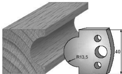
SP-Messer/Blade = Art.-Nr./Item no. 36118 HS-Messer/Blade = Art.-Nr./Item no. 36418 Abweiser/Deflector = Art.-Nr./Item no. 37118
