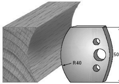
SP-Messer/Blade = Art.-Nr./Item no. 38553 HS-Messer/Blade = Art.-Nr./Item no. 36553 Abweiser/Deflector = Art.-Nr./Item no. 39553
