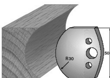
SP-Messer/Blade = Art.-Nr./Item no. 38541 HS-Messer/Blade = Art.-Nr./Item no. 36541 Abweiser/Deflector = Art.-Nr./Item no. 39541
