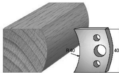
SP-Messer/Blade = Art.-Nr./Item no. 3608 HS-Messer/Blade = Art.-Nr./Item no. 36308 Abweiser/Deflector = Art.-Nr./Item no. 3708
