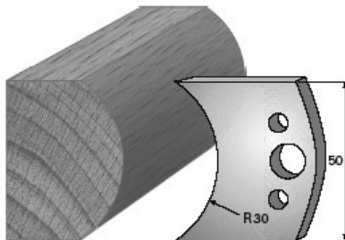
SP-Messer/Blade = Art.-Nr./Item no. 38547 HS-Messer/Blade = Art.-Nr./Item no. 36547 Abweiser/Deflector = Art.-Nr./Item no. 39547
