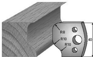
SP-Messer/Blade = Art.-Nr./Item no. 3649 HS-Messer/Blade = Art.-Nr./Item no. 36349 Abweiser/Deflector = Art.-Nr./Item no. 3749
