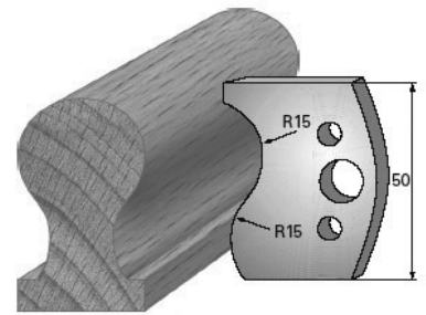
SP-Messer/Blade = Art.-Nr./Item no. 38514 HS-Messer/Blade = Art.-Nr./Item no. 36514 Abweiser/Deflector = Art.-Nr./Item no. 39514
