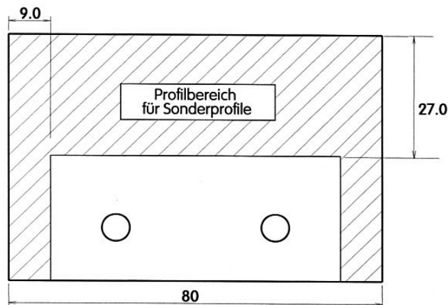
HS-Messer/Blade = Art.-Nr./Item no. 80500 Abweiser Blankett/Deflector Blank = Art.-Nr./Item no. 81500
