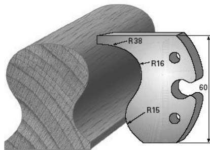
SP-Messer/Blade = Art.-Nr./Item no. 60004 HS-Messer/Blade = Art.-Nr./Item no. 62004 Abweiser/Deflector = Art.-Nr./Item no. 61004
