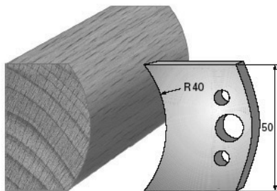
SP-Messer/Blade = Art.-Nr./Item no. 38555 HS-Messer/Blade = Art.-Nr./Item no. 36555 Abweiser/Deflector = Art.-Nr./Item no. 39555
