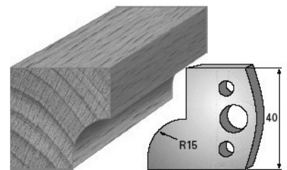
SP-Messer/Blade = Art.-Nr./Item no. 3657 HS-Messer/Blade = Art.-Nr./Item no. 36357 Abweiser/Deflector = Art.-Nr./Item no. 3757
