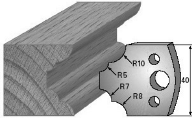
SP-Messer/Blade = Art.-Nr./Item no. 3622 HS-Messer/Blade = Art.-Nr./Item no. 36322 Abweiser/Deflector = Art.-Nr./Item no. 3722
