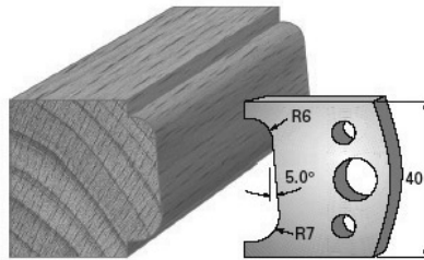
SP-Messer/Blade = Art.-Nr./Item no. 3602 HS-Messer/Blade = Art.-Nr./Item no. 36302 Abweiser/Deflector = Art.-Nr./Item no. 3702
