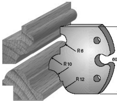
SP-Messer/Blade = Art.-Nr./Item no. 60001 HS-Messer/Blade = Art.-Nr./Item no. 62001 Abweiser/Deflector = Art.-Nr./Item no. 61001
