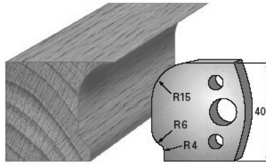
SP-Messer/Blade = Art.-Nr./Item no. 3647 HS-Messer/Blade = Art.-Nr./Item no. 36347 Abweiser/Deflector = Art.-Nr./Item no. 3747
