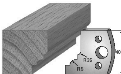
SP-Messer/Blade = Art.-Nr./Item no. 3620 HS-Messer/Blade = Art.-Nr./Item no. 36320 Abweiser/Deflector = Art.-Nr./Item no. 3720
