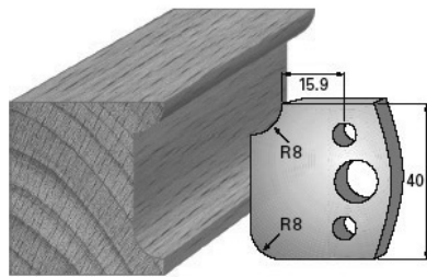
SP-Messer/Blade = Art.-Nr./Item no. 36174 HS-Messer/Blade = Art.-Nr./Item no. 36474 Abweiser/Deflector = Art.-Nr./Item no. 37174
