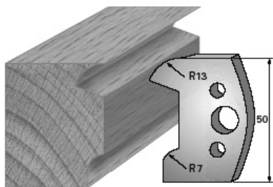
SP-Messer/Blade = Art.-Nr./Item no. 38518 HS-Messer/Blade = Art.-Nr./Item no. 36518 Abweiser/Deflector = Art.-Nr./Item no. 39518
