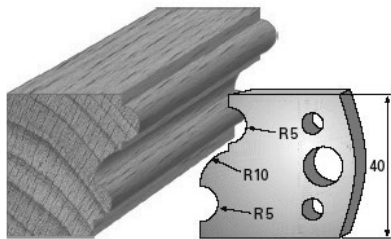
SP-Messer/Blade = Art.-Nr./Item no. 3652 HS-Messer/Blade = Art.-Nr./Item no. 36352 Abweiser/Deflector = Art.-Nr./Item no. 3752
