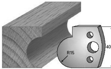
SP-Messer/Blade = Art.-Nr./Item no. 3665 HS-Messer/Blade = Art.-Nr./Item no. 36365 Abweiser/Deflector = Art.-Nr./Item no. 3765
