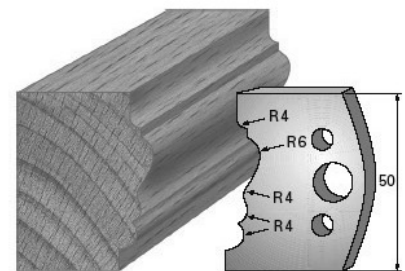
SP-Messer/Blade = Art.-Nr./Item no. 38511 HS-Messer/Blade = Art.-Nr./Item no. 36511 Abweiser/Deflector = Art.-Nr./Item no. 39511
