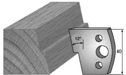
SP-Messer/Blade = Art.-Nr./Item no. 3627 HS-Messer/Blade = Art.-Nr./Item no. 36327 Abweiser/Deflector = Art.-Nr./Item no. 3727
