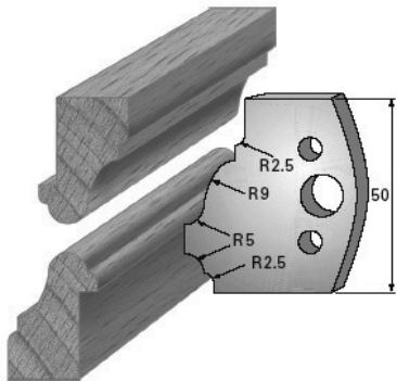
SP-Messer/Blade = Art.-Nr./Item no. 38558 HS-Messer/Blade = Art.-Nr./Item no. 36558 Abweiser/Deflector = Art.-Nr./Item no. 39558
