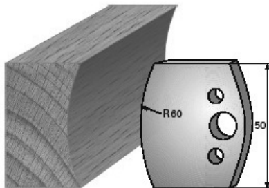
SP-Messer/Blade = Art.-Nr./Item no. 38574 HS-Messer/Blade = Art.-Nr./Item no. 36574 Abweiser/Deflector = Art.-Nr./Item no. 39574
