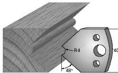
SP-Messer/Blade = Art.-Nr./Item no. 3680 HS-Messer/Blade = Art.-Nr./Item no. 36380 Abweiser/Deflector = Art.-Nr./Item no. 3780
