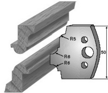
SP-Messer/Blade = Art.-Nr./Item no. 38542 HS-Messer/Blade = Art.-Nr./Item no. 36542 Abweiser/Deflector = Art.-Nr./Item no. 39542
