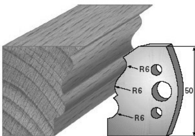
SP-Messer/Blade = Art.-Nr./Item no. 38509 HS-Messer/Blade = Art.-Nr./Item no. 36509 Abweiser/Deflector = Art.-Nr./Item no. 39509
