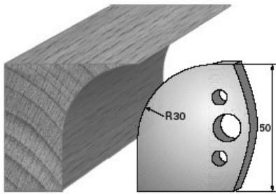
SP-Messer/Blade = Art.-Nr./Item no. 38563 HS-Messer/Blade = Art.-Nr./Item no. 36563 Abweiser/Deflector = Art.-Nr./Item no. 39563
