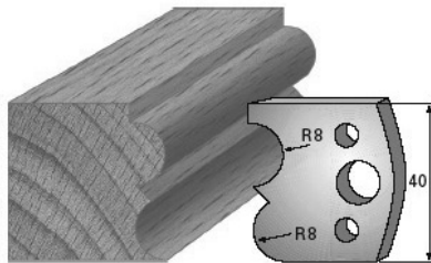
SP-Messer/Blade = Art.-Nr./Item no. 3628 HS-Messer/Blade = Art.-Nr./Item no. 36328 Abweiser/Deflector = Art.-Nr./Item no. 3728
