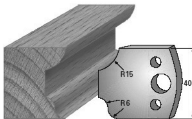
SP-Messer/Blade = Art.-Nr./Item no. 3644 HS-Messer/Blade = Art.-Nr./Item no. 36344 Abweiser/Deflector = Art.-Nr./Item no. 3744
