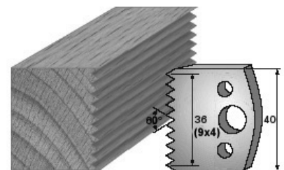
SP-Messer/Blade = Art.-Nr./Item no. 36117 HS-Messer/Blade = Art.-Nr./Item no. 36417 Abweiser/Deflector = Art.-Nr./Item no. 37117
