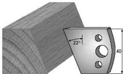
SP-Messer/Blade = Art.-Nr./Item no. 3601 HS-Messer/Blade = Art.-Nr./Item no. 36301 Abweiser/Deflector = Art.-Nr./Item no. 3701
