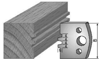
SP-Messer/Blade = Art.-Nr./Item no. 3675 HS-Messer/Blade = Art.-Nr./Item no. 36375 Abweiser/Deflector = Art.-Nr./Item no. 3775
