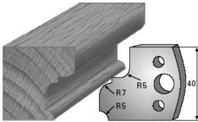
SP-Messer/Blade = Art.-Nr./Item no. 3682 HS-Messer/Blade = Art.-Nr./Item no. 36382 Abweiser/Deflector = Art.-Nr./Item no. 3782
