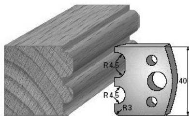
SP-Messer/Blade = Art.-Nr./Item no. 3607 HS-Messer/Blade = Art.-Nr./Item no. 36307 Abweiser/Deflector = Art.-Nr./Item no. 3707
