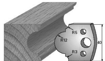
SP-Messer/Blade = Art.-Nr./Item no. 3618 HS-Messer/Blade = Art.-Nr./Item no. 36318 Abweiser/Deflector = Art.-Nr./Item no. 3718
