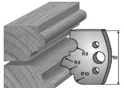
SP-Messer/Blade = Art.-Nr./Item no. 38520 HS-Messer/Blade = Art.-Nr./Item no. 36520 Abweiser/Deflector = Art.-Nr./Item no. 39520
