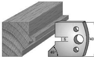
SP-Messer/Blade = Art.-Nr./Item no. 3683 HS-Messer/Blade = Art.-Nr./Item no. 36383 Abweiser/Deflector = Art.-Nr./Item no. 3783
